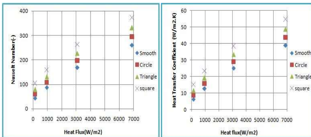
Figure (13) (h), (Nu) with different heat flux for all ribs type (Reynolds number 10460).
