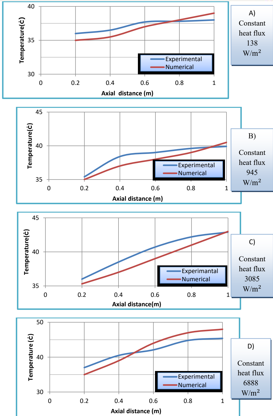
Figure (5) Comparison of experimental and numerical data.
