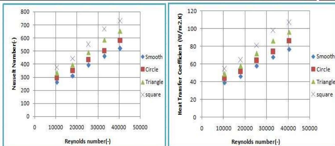
Figure (12) (h), (Nu) with Reynolds number for all ribs type (constant heat flux 6888 W/m² ).
