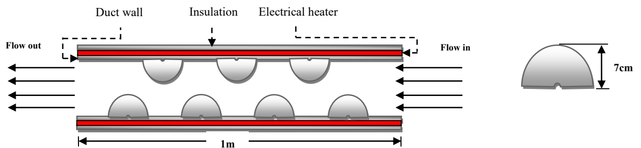
➤ Duct with semicircle ribs
