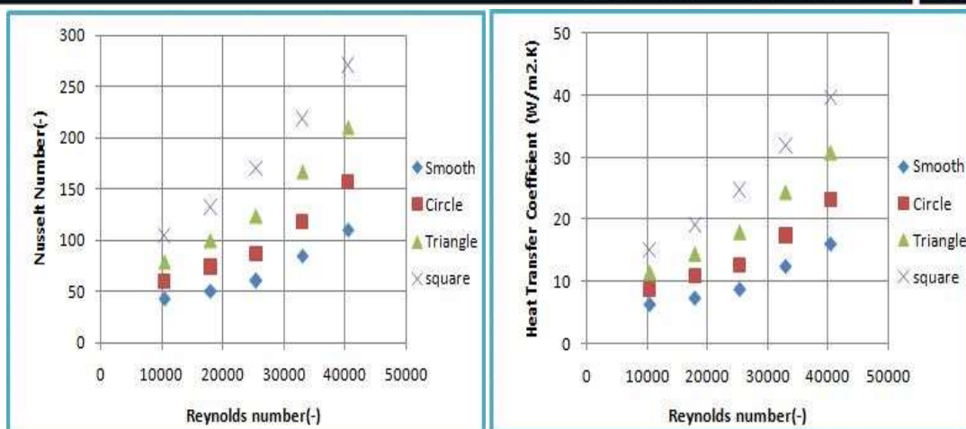
Figure (9) (h), (Nu) with Reynolds number for all ribs type (constant heat flux 138 W/m 2 ).
